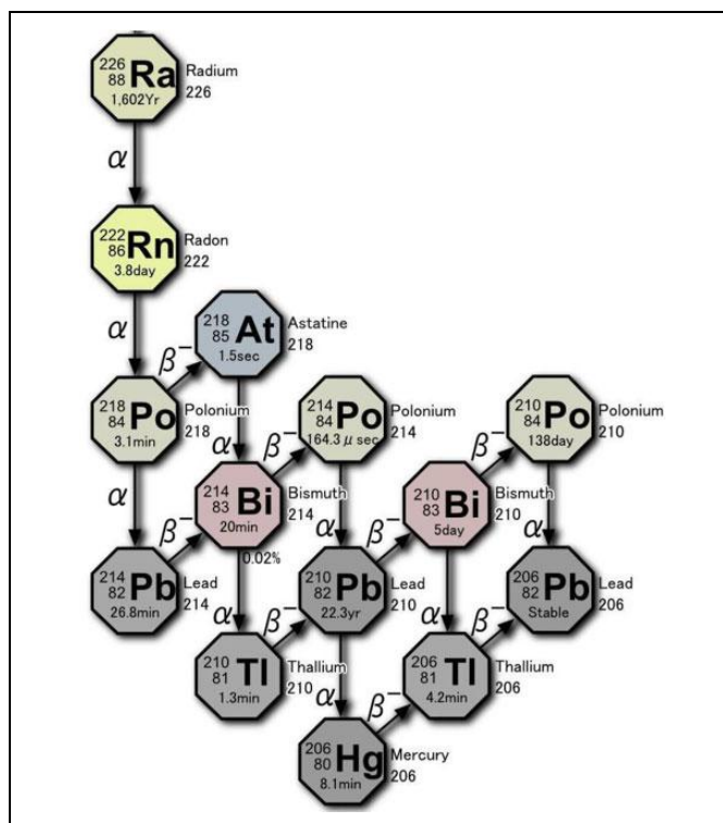
Figure 1. Radioactive decay chain of ^{222}\text{Rn} .
